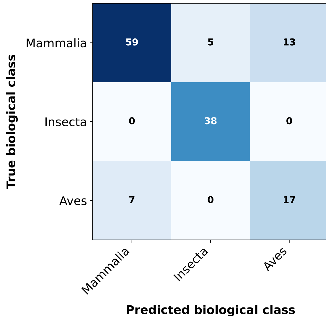
(b) Class-trained GCN
