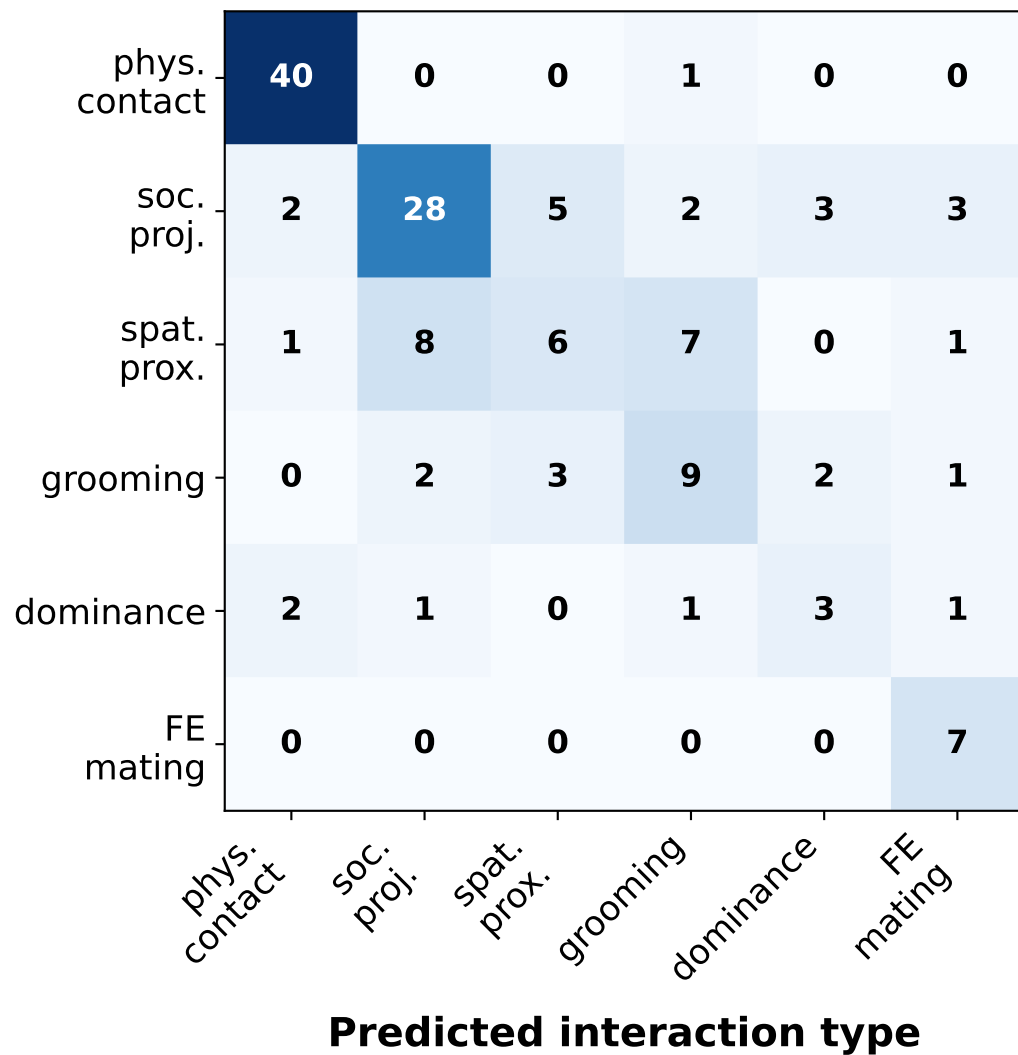
(a) Interaction-trained GCN
